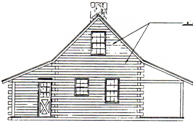
LEFT SIDE ELEVATION SCALE: 1/4" = 1'-0"
