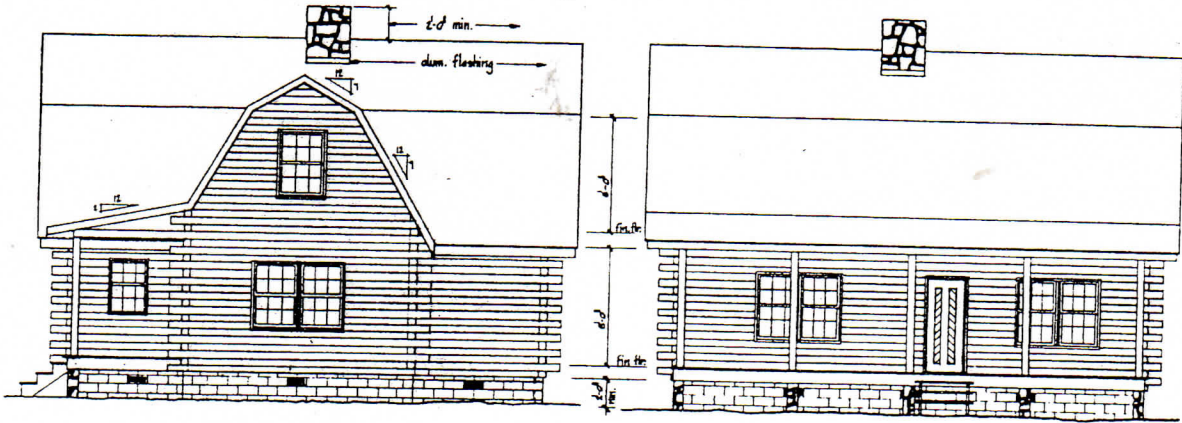
REAR ELEVATION 3/4" = 1'-0"
